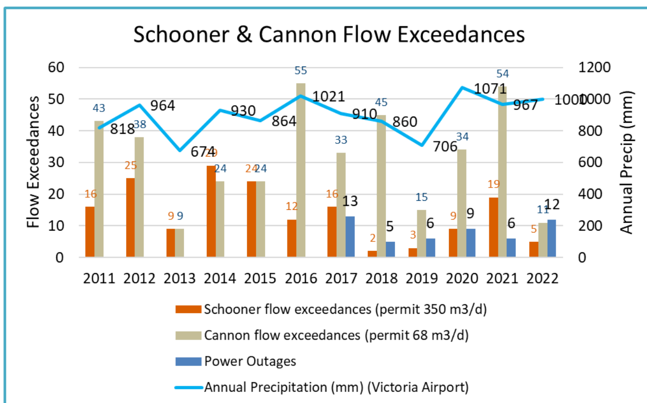
Figure 8: Schooner and Cannon Wastewater Treatment Plant (WWTP) Flow Exceedances
