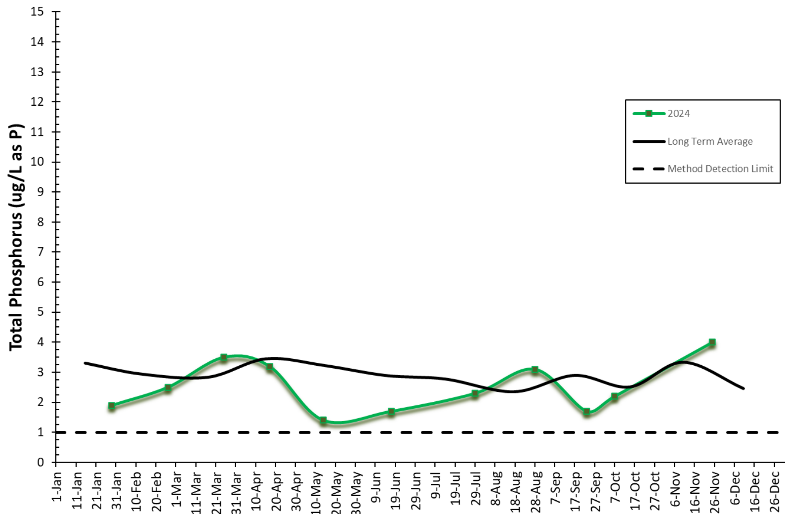
Figure 24 Total Phosphorus in Sooke Lake Reservoir, North Basin, 1 m depth (SOL-04-01)
