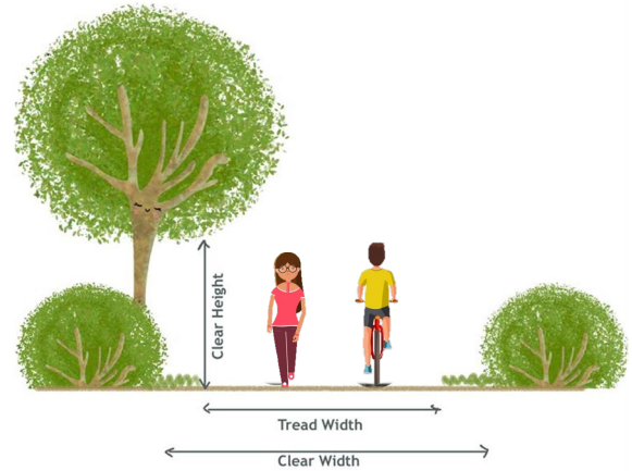
Figure 5.2 Trail Clearance Design Parameters
