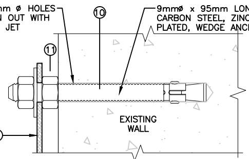
WEDGE ANCHOR DETAIL
