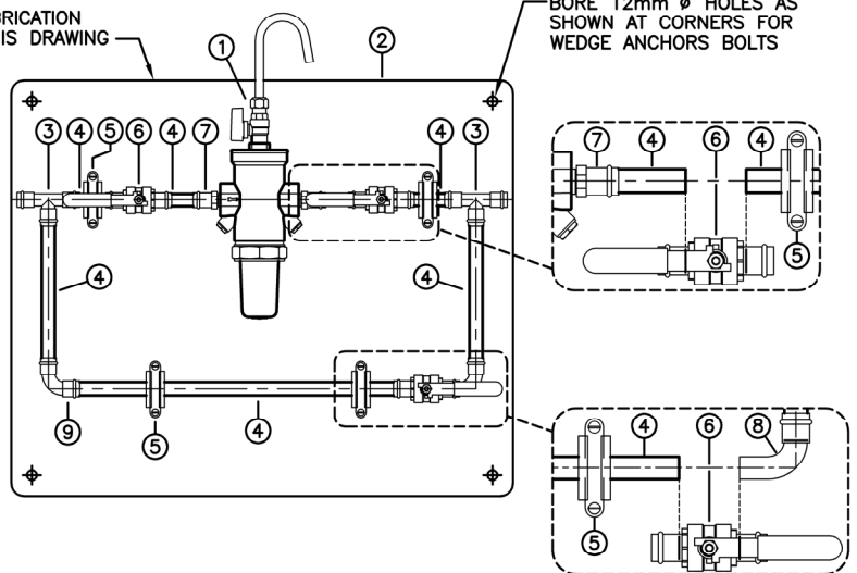
STRAINER ASSEMBLY DETAIL
