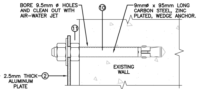
WEDGE ANCHOR DETAIL
