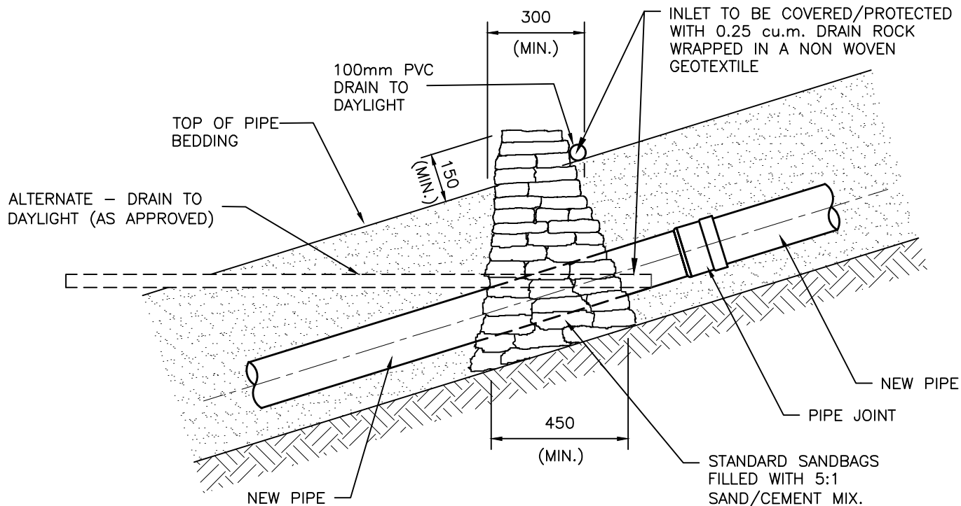
SIDE VIEW
